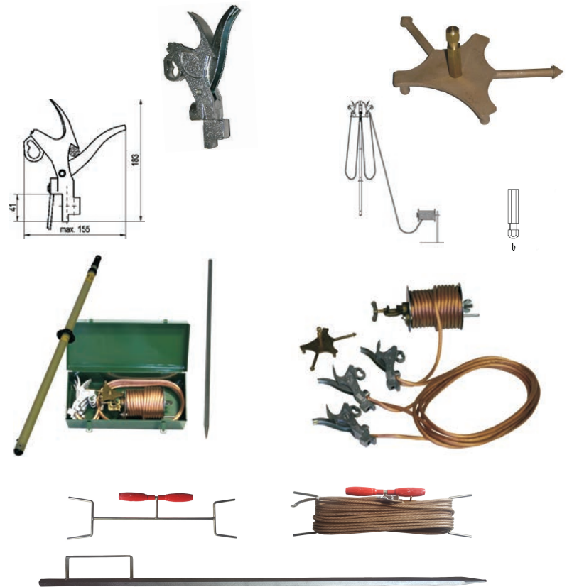
KÖF-KJ-8901/1 phase clamp
